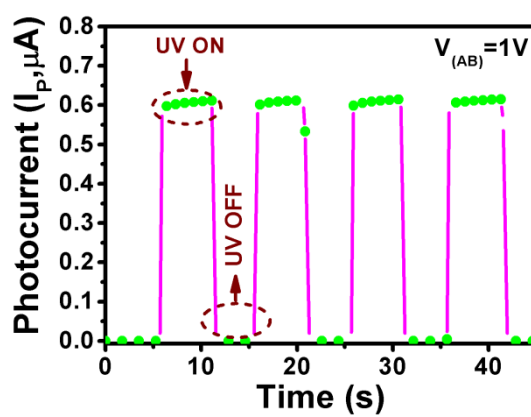
Figure S1. Time response of the nanoPCDs under UV light illumination ( 1 \mu\text{Wcm}^{-2} ) under a bias of 1 V.
