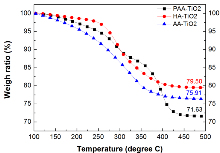
Figure S1 TGA thermograms of different surface-modified TiO 2
