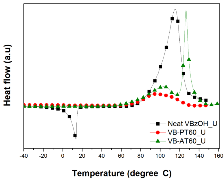
Figure S5 DSC thermograms of uncured sample upon heating
