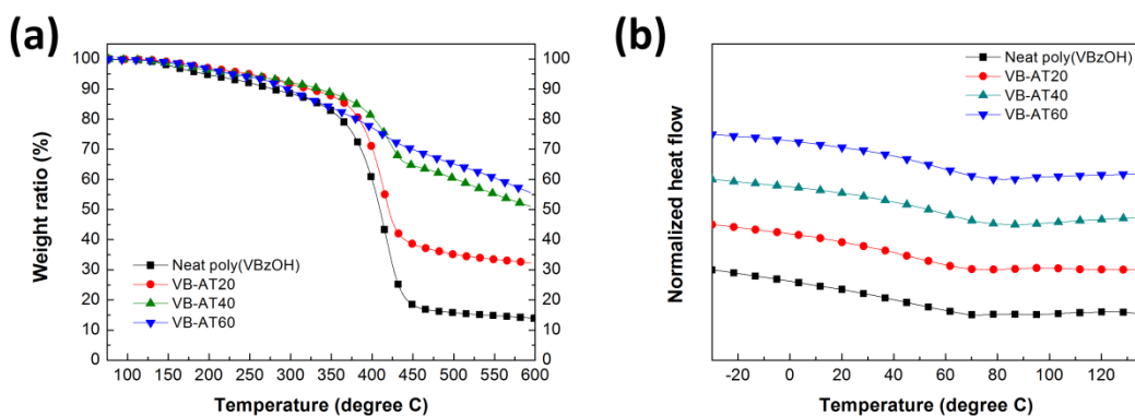
Figure S4 (a)TGA thermograms of AA-TiO 2 /polyVBzOH (VB-AT series) nanocomposite, (b) DSC thermograms of AA-TiO 2 /polyVBzOH (VB-AT series) nanocomposite
