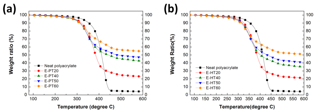
Figure S3 TGA thermograms of (a) PAA-TiO 2 /polyacrylate (E-PT series), (b) HA-TiO 2 /polyacrylate (E-HT series)
