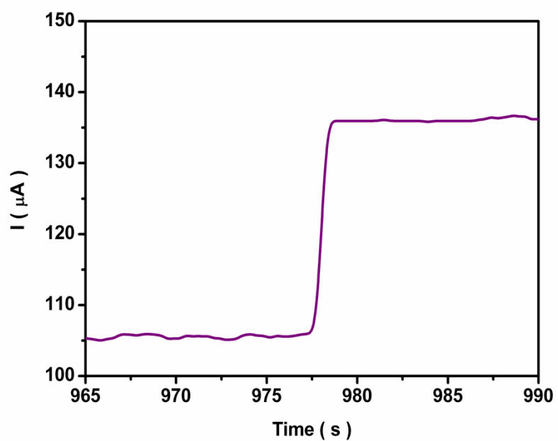
Fig. S4 The enlargement of one step addition of \text{H}_2\text{O}_2 in Fig. 9(A)
