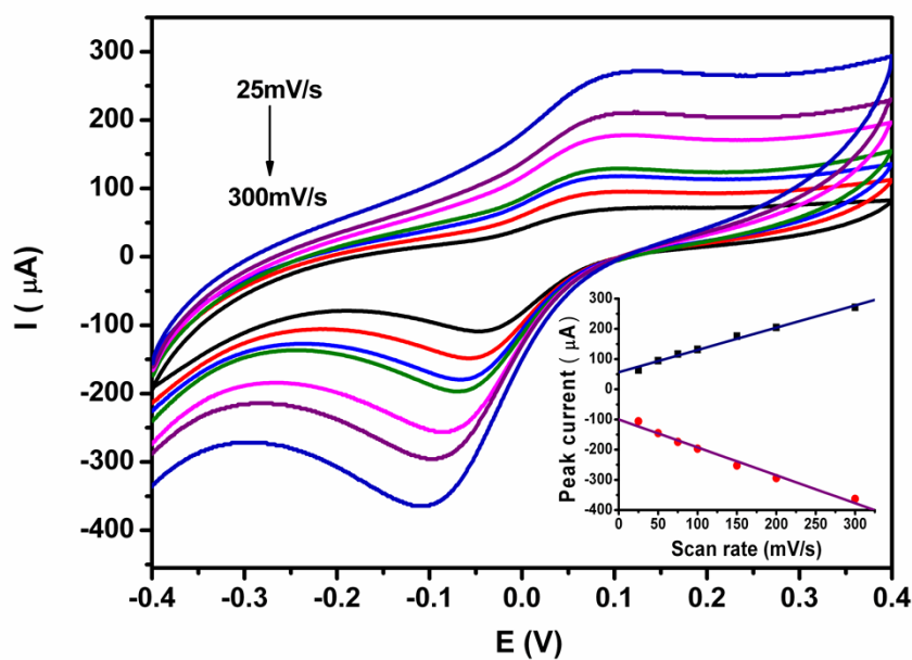
Fig. S2 Cyclic voltammograms of {IL-GR/s-PANI} 8 multilayer film in PBS buffers
