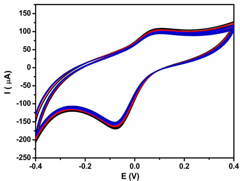
Fig. S3 Cyclic voltammograms of {IL-GR/s-PANI} 8 modified electrode in 0.1 M PBS buffer solution, pH 7.0 upon repeated cyclic potential scan. Scan rate was 100 mV/s.
