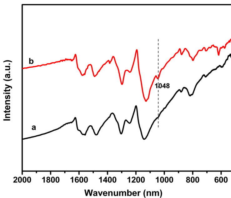
Fig. S1 FTIR spectra of PANI (a), s-PANI (b).
