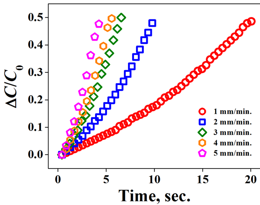
Fig. S2 Slopes in capacitance change ratio under various loading speeds with fixed maximum loading pressure of \sim 0.8 Mpa.
