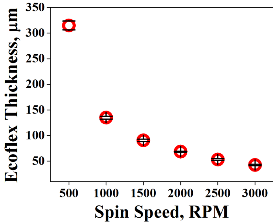
Fig. S1 Thickness variations of Ecoflex layer as a function of spin speed.
