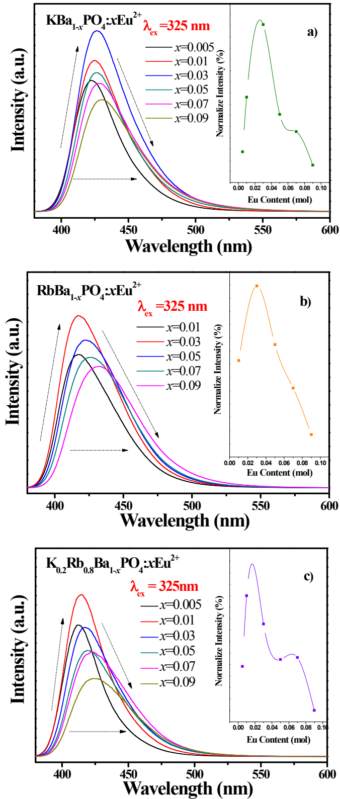
Fig. S1. PL spectra of the a) \text{KBa}_{1-x}\text{PO}_4:x\text{Eu}^{2+} , b) \text{RbBa}_{1-x}\text{PO}_4:x\text{Eu}^{2+} , c) \text{K}_{0.2}\text{Rb}_{0.8}\text{Ba}_{1-x}\text{PO}_4:x\text{Eu}^{2+} phosphors and the inset shows the Eu content dependent PL intensity.
