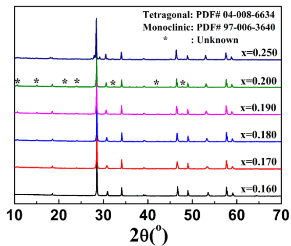
Figure S1 X-ray diffraction patterns of CBM ceramics in the x range of 0.16-0.25
