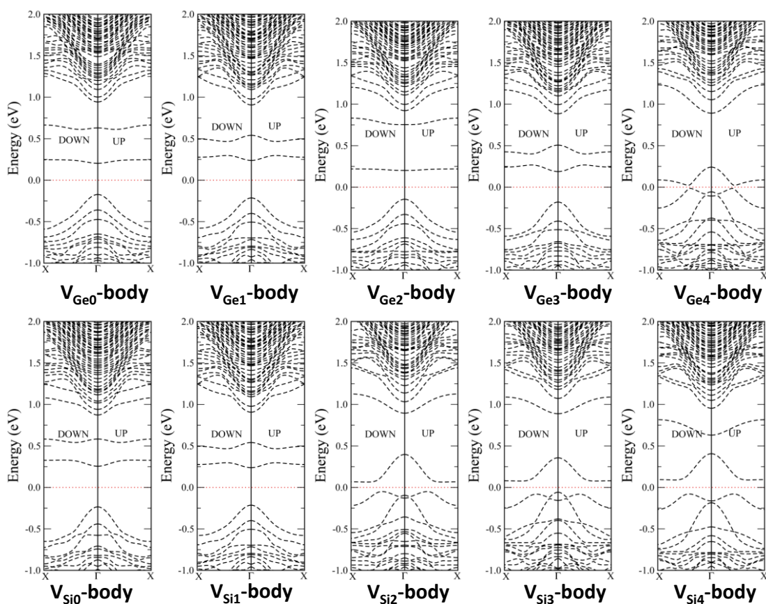
Figure S1 Computed band structures of the random-distributed triangular-prism (RTP) Si/Ge NWs with Ge and Si single vacancy in the body.
