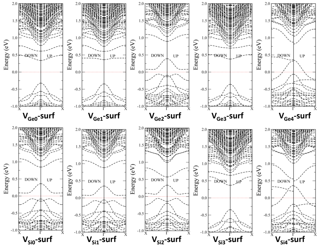
Figure S2 Computed band structures of the random-distributed triangular-prism (RTP) Si/Ge NWs with Ge and Si single vacancy on the surface.
