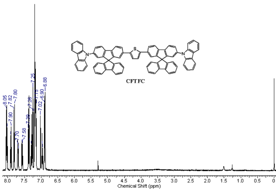
Fig. S5 1 HNMR spectrum of CFTFC.
