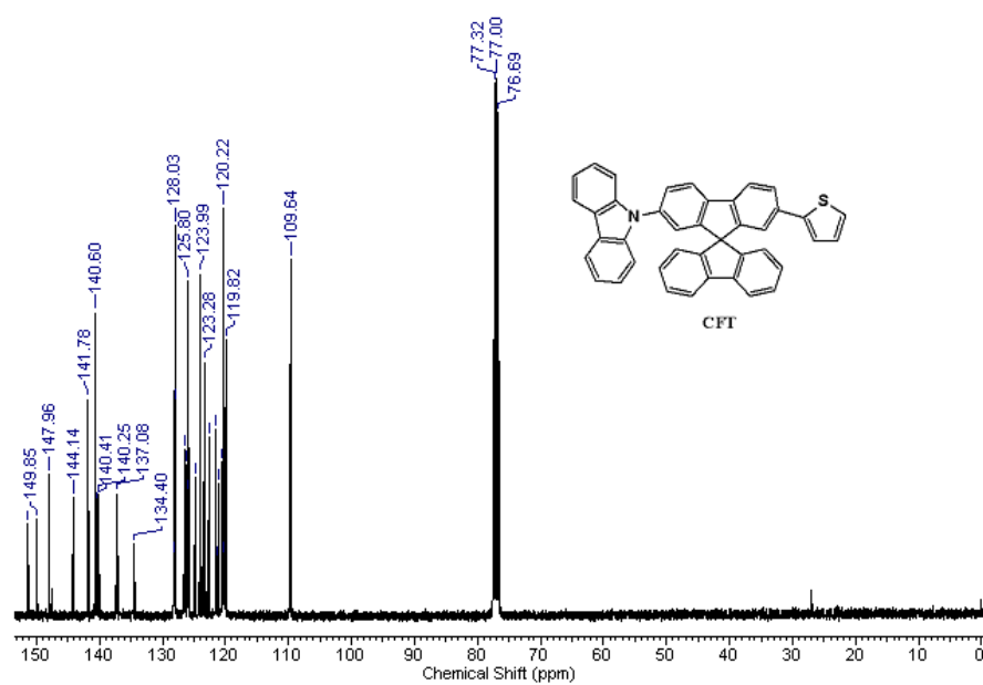
Fig. S2 13 CNMR spectrum of CFT.
