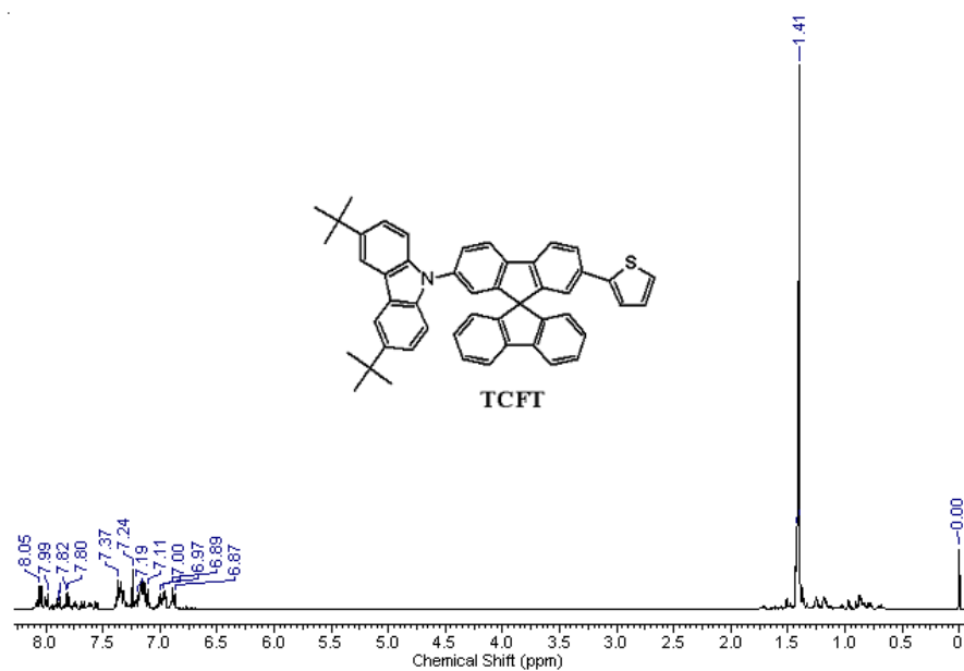
Fig. S3 1 HNMR spectrum of TCFT.
