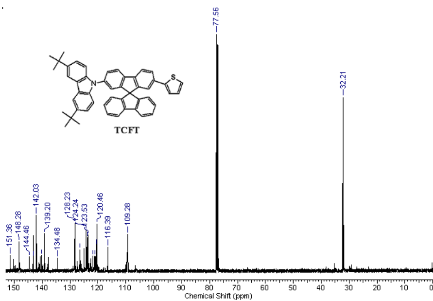
Fig. S4 13 CNMR spectrum of TCFT.
