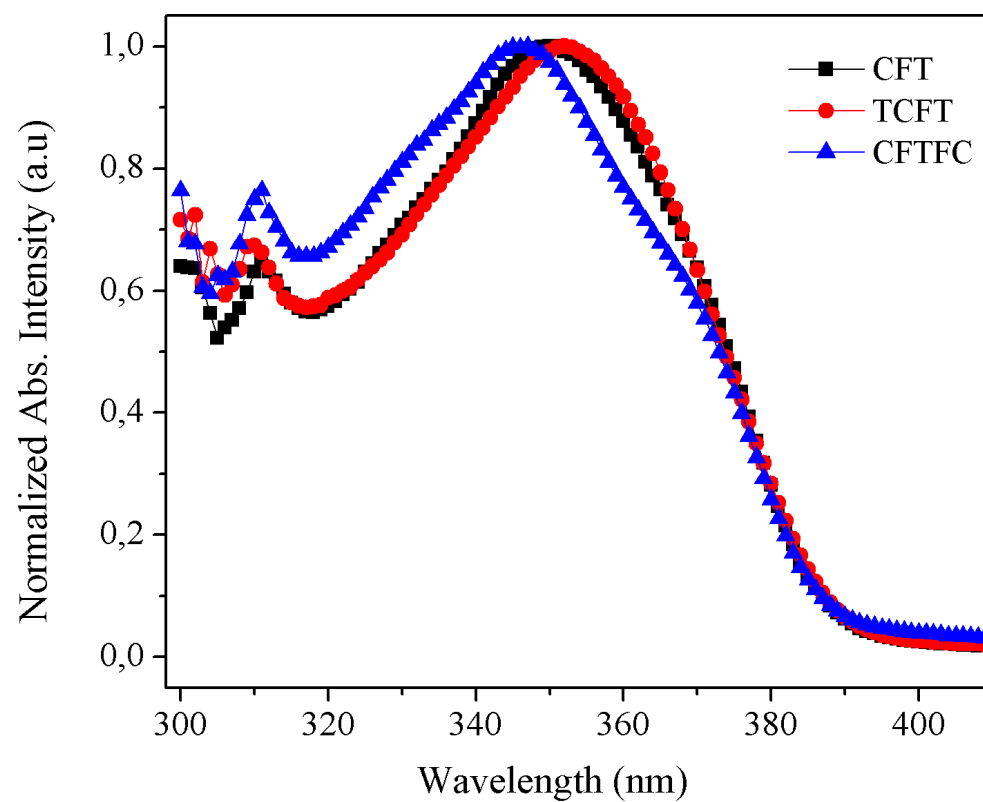
Fig. S7 Normalized UV-Vis absorption spectra of CFT, TCFT and CFTFC thin films.
