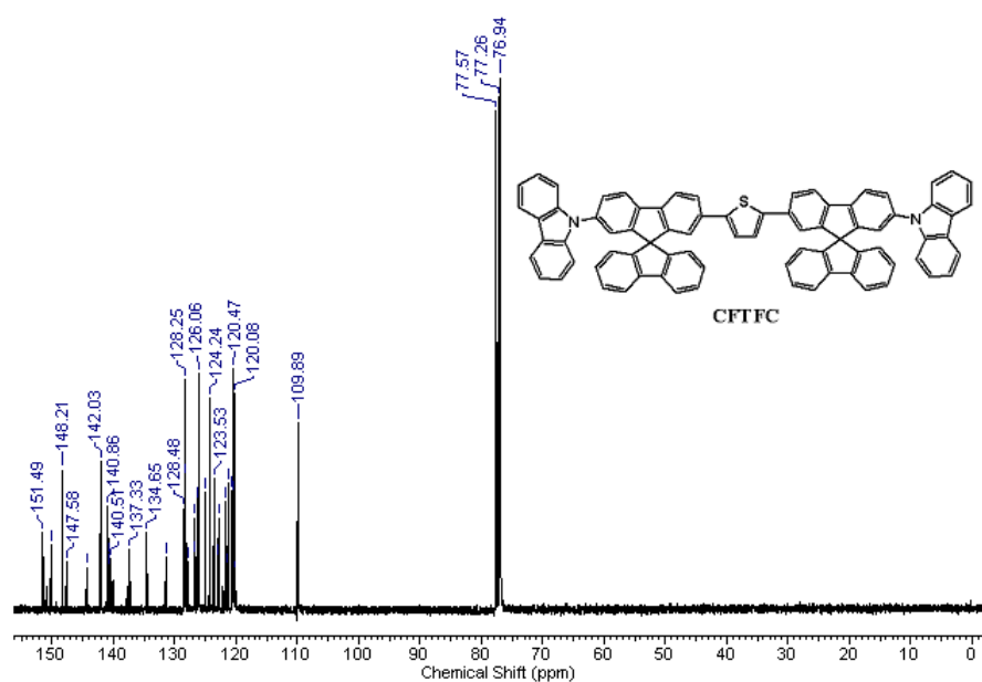
Fig. S6 ^{13}\text{C} NMR spectrum of CFTFC.
