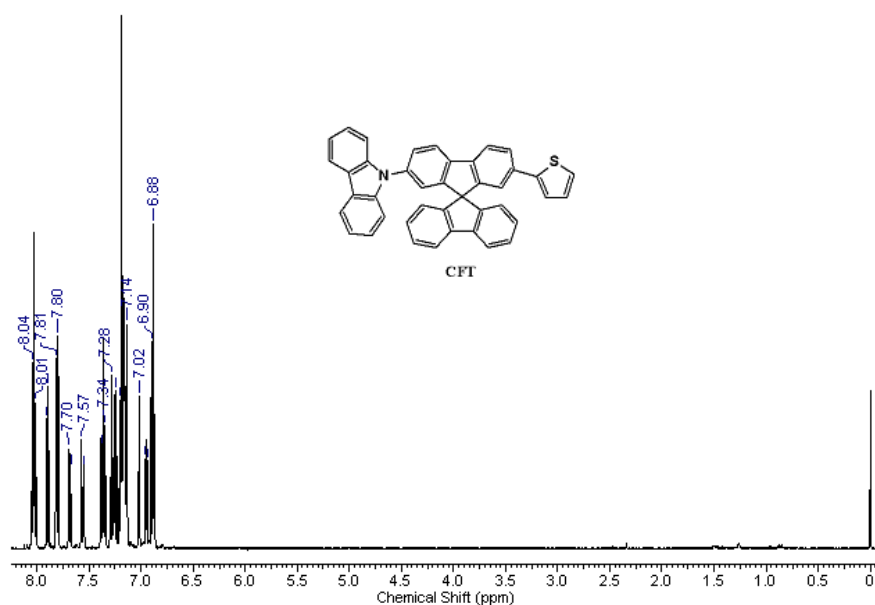
Fig. S1 1 H NMR spectrum of CFT.
