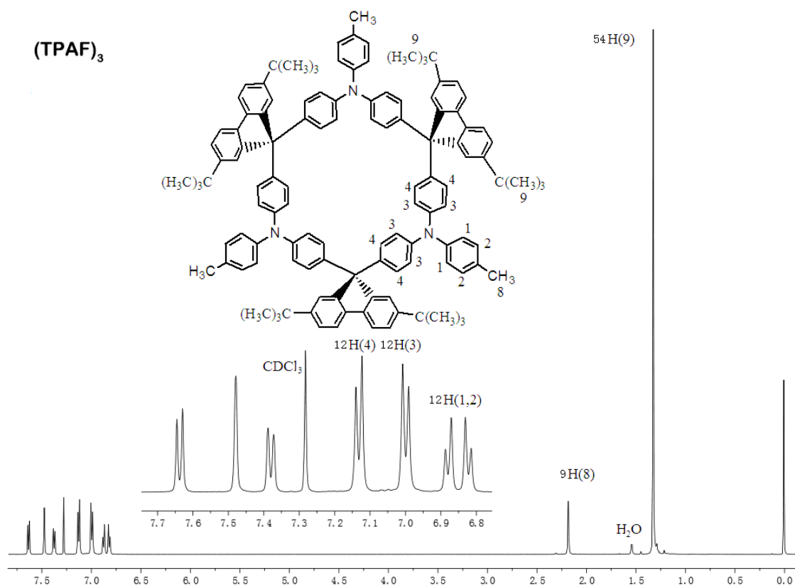
Fig. S1 ^1\text{H} spectra of TPAF-OH and (TPAF) 3 .
