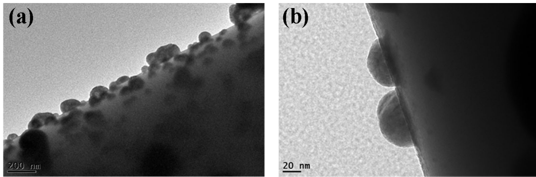
Figure S1. TEM images of \text{SiO}_2@\text{Bi}_2\text{O}_3 composite fibers calinated at 400 °C, which show that \text{Bi}_2\text{O}_3 nanoparticles only distribute on the surface of \text{SiO}_2 fibers.
