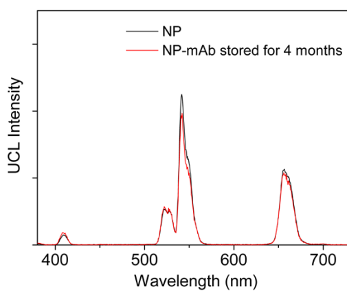
Fig S2: The luminescence spectra of the UCL nanoparticle (NP) and UCL particle-mAb (NP-mAb) conjugate.
