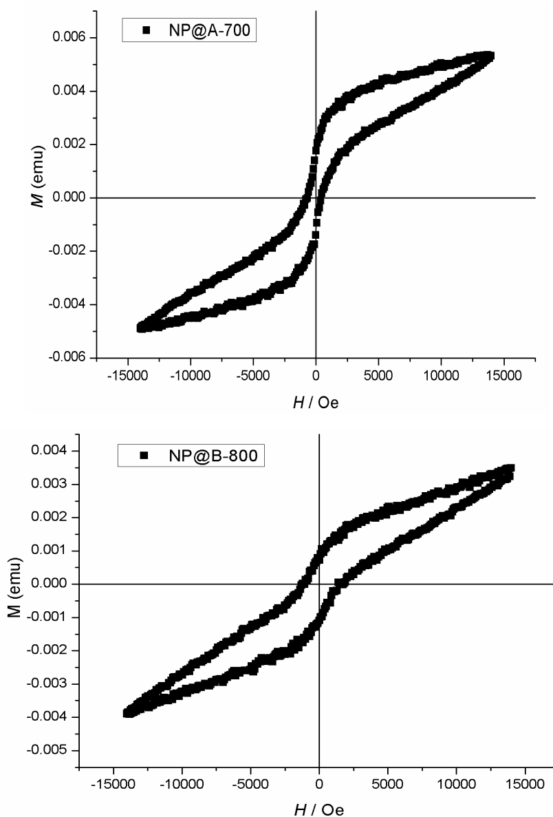
Fig. S1 Hysteresis loops of NP@A-700 (Top) and NP@B-800 (Bottom) measured at 100 K.
