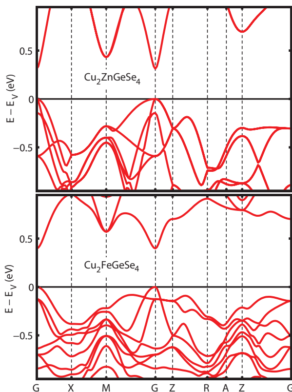
Fig. 1 Calculated band structures of stannite-type \text{Cu}_2\text{ZnGeSe}_4 (top) and kesterite-type \text{Cu}_2\text{FeGeSe}_4 (bottom), showing the different configurations at the Gamma-point (G).
