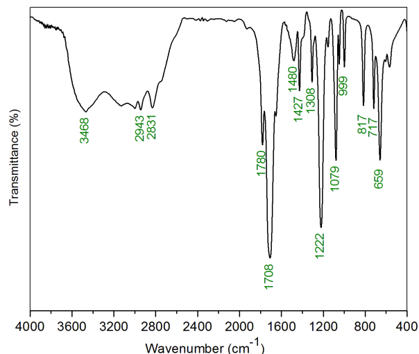
Figure S2. FT-IR spectra of N-Hydroxysuccinimide
