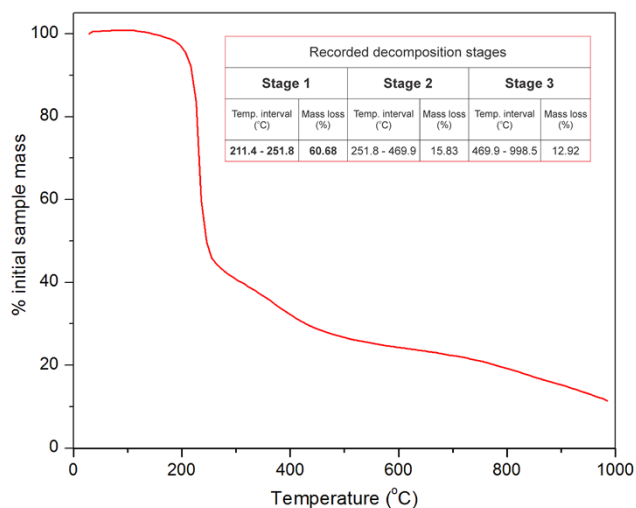
Figure S1. Thermal decomposition of unprocessed N-Hydroxysuccinimide
