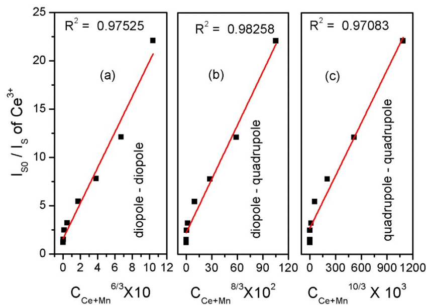
Figure S1. Dependence of I_{S0} / I_S of Ce^{3+} on C^{6/3} , C^{8/3} and C^{10/3}
