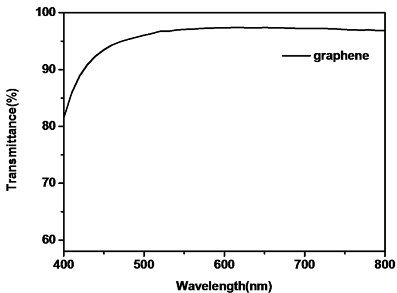
Fig. S2 Optical transmittance spectra of graphene on PET substrate
