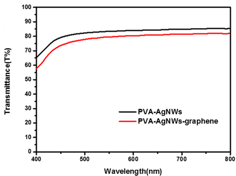
Fig. S1 Optical transmittance spectra of PVA-AgNWs film and PVA encapsulated AgNWs-graphene hybrid film on PET substrate
