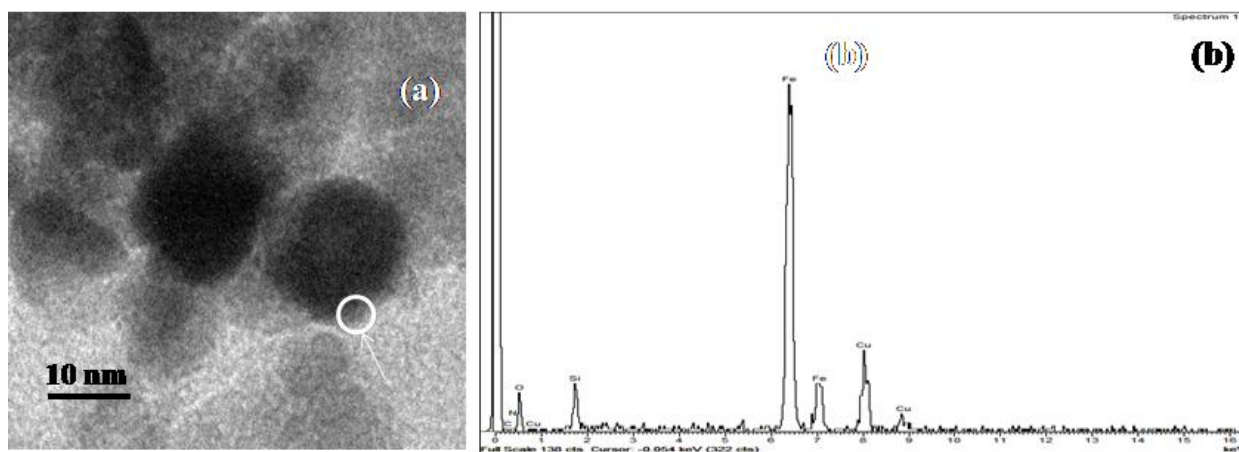
Figure S1: Higher magnification of TEM image (a) and corresponding EDX (b) of AMNPs
